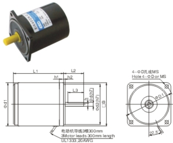
3~40W感应电动机光机外形图 3~40W Induction bare motor dimension
