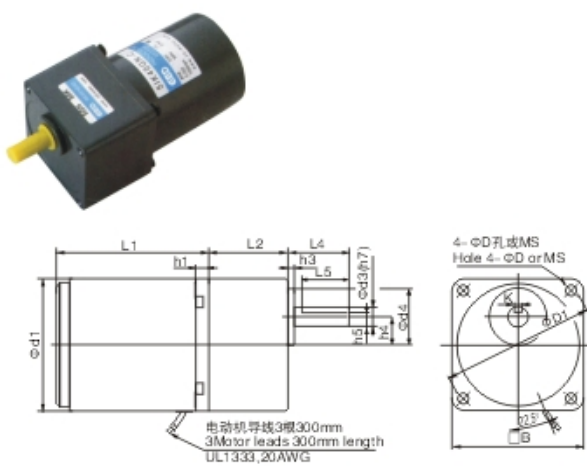
3~40W感应减速电动机整机外形图 3~40W Induction gear motor dimension
